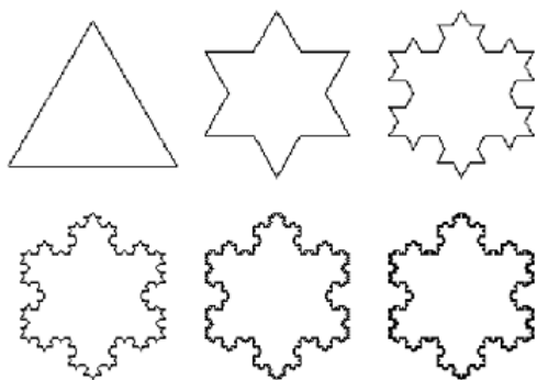
▲ Figure 3. Design fractals with similarity dimension
